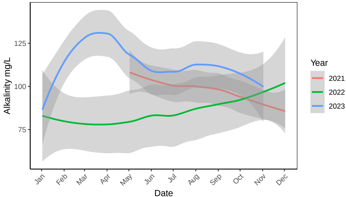
B2 Raceway 2 Alkalinity mg/L Monthly Mean
